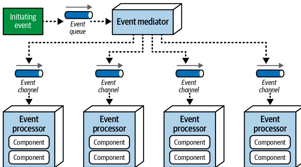
Figure 15-25. Mediator topology
