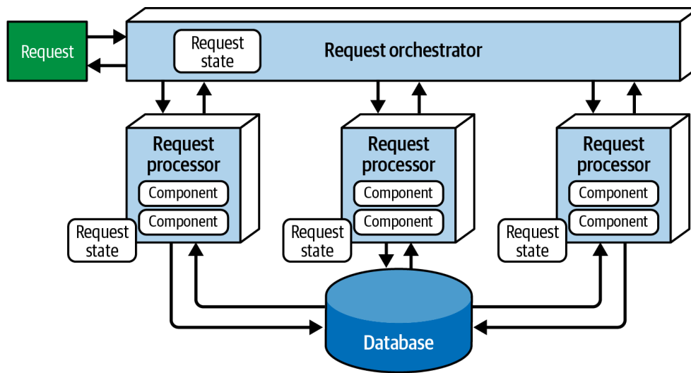
Figure 15-1. Request-based model
