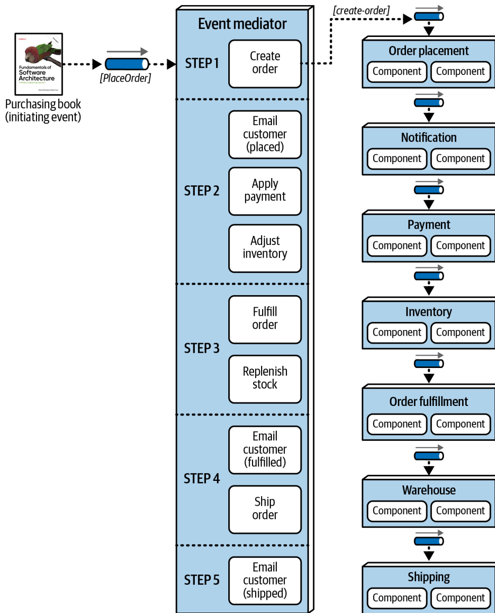
Figure 15-28. Step 1 of the mediator example
